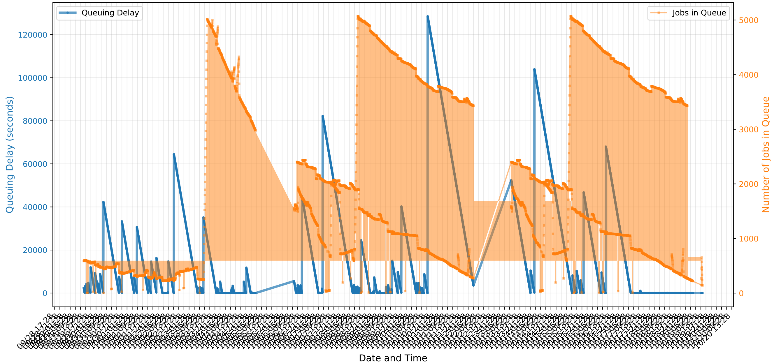
UGE Cluster Queuing Delay Over Time for 64 Core Jobs
